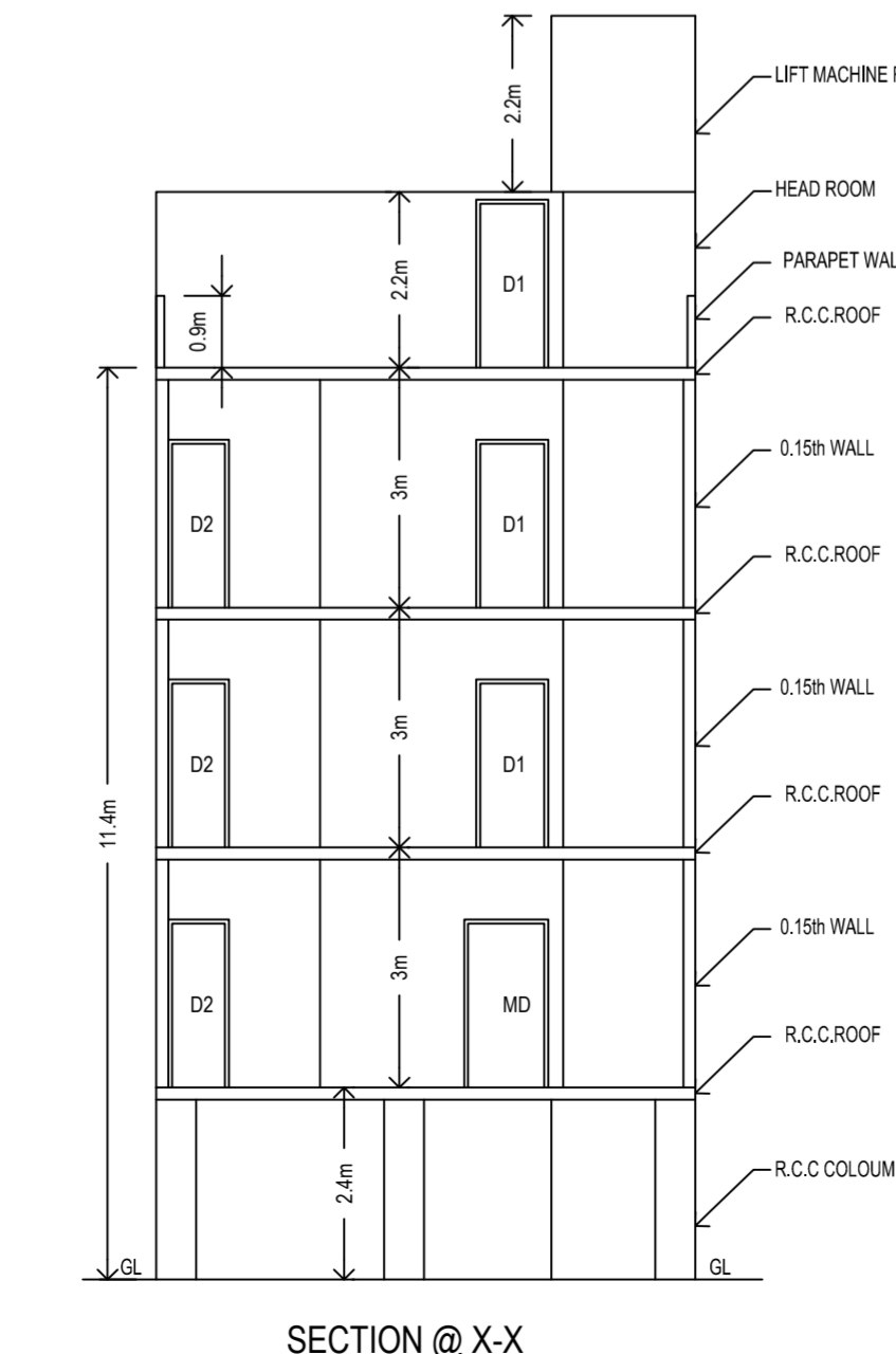
SECTION @ X-X
